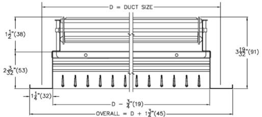
Adjustable double deflection supply grille
