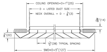
Border: 6 Beveled Frame Surface Mount
