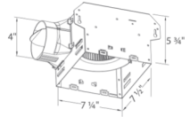
DeltaBreez ITG80
