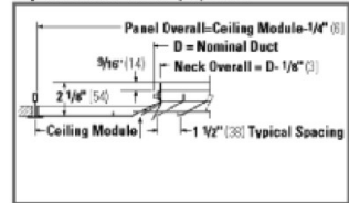
Type 3P Lay-In Inverted Tee 1" (25) Panel
