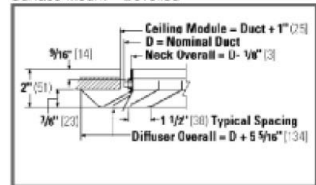
Type 6 Surface Mount — Beveled
